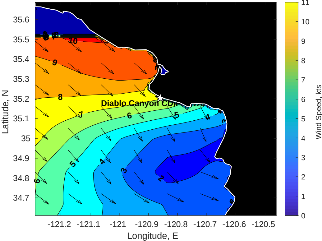
Winds (kts) for Diablo Canyon CDIP SWAN at 19-Nov-2025 18:00:00
