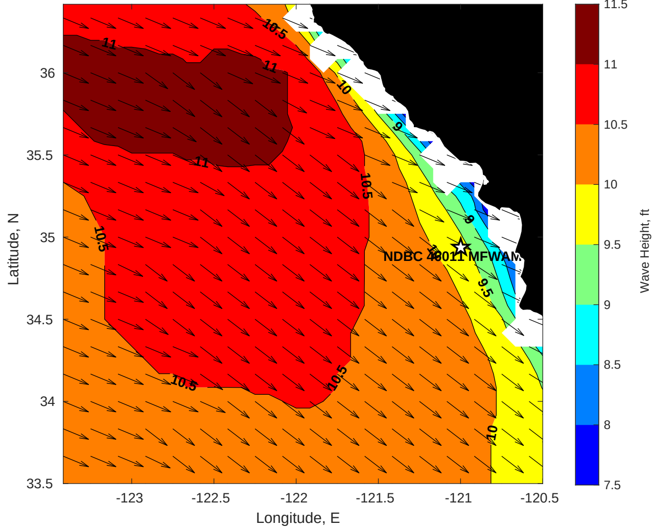
WAM Wave Height (ft) for NDBC 46011 MFWAM at 24-Nov-2025 09:00:00
