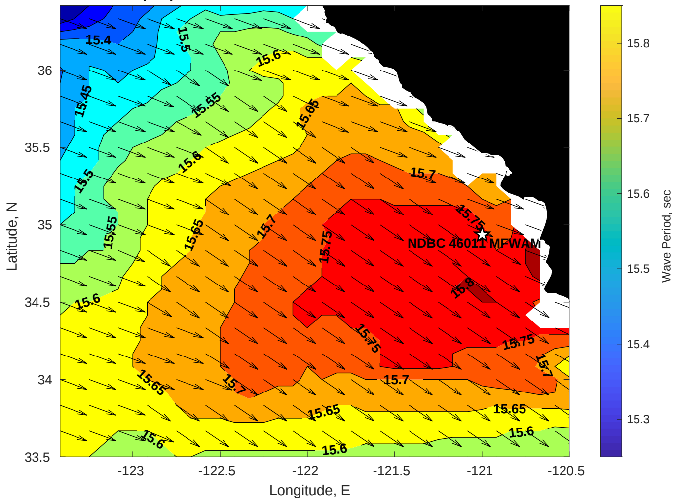
WAM Wave Period (sec) for NDBC 46011 MFWAM at 24-Nov-2025 09:00:00
