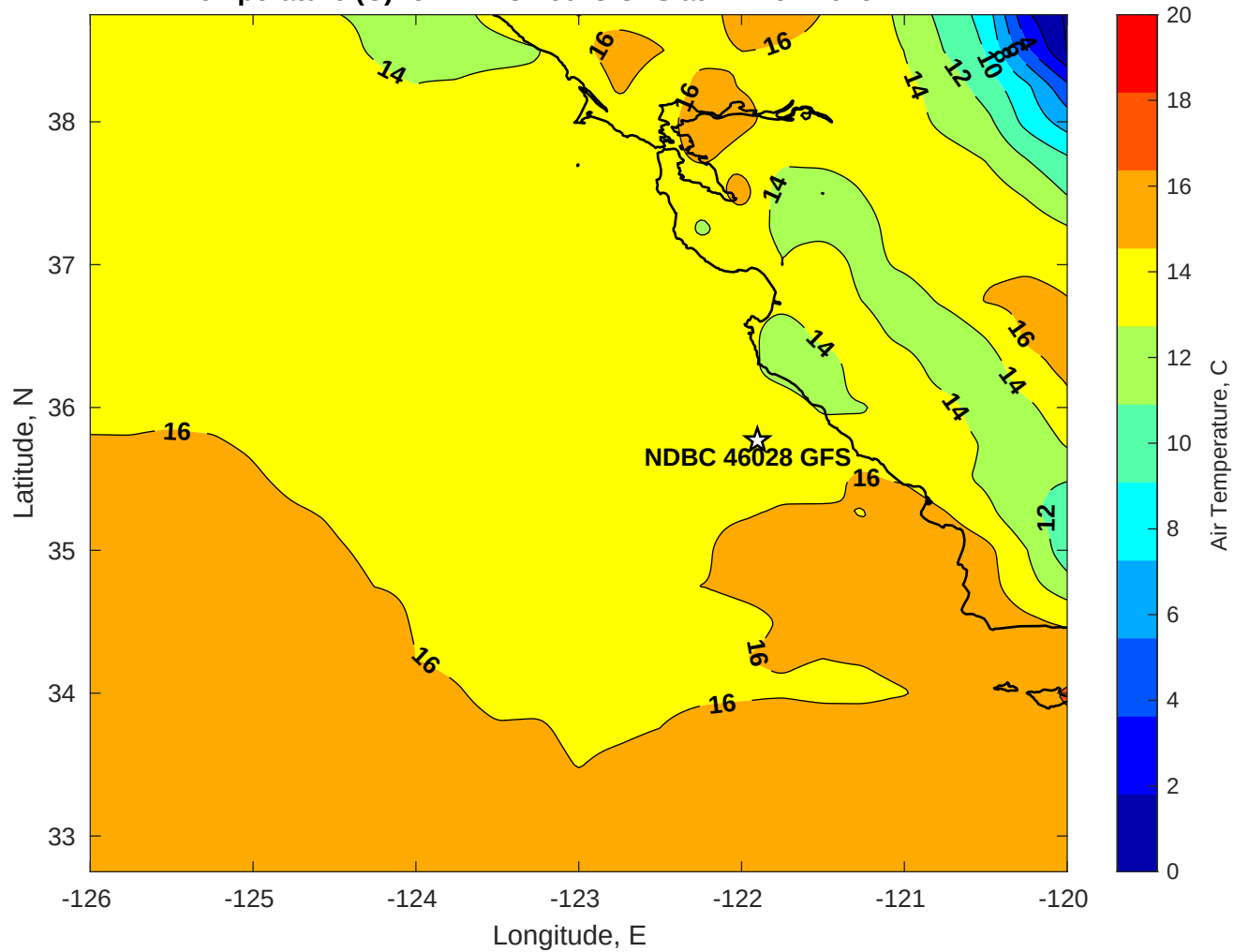
Air Temperature (C) for NDBC 46028 GFS at 21-Nov-2025
