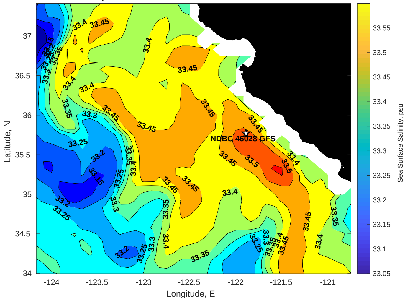
Surface Salinity for NDBC 46028 GFS at 19-Nov-2025 00:00:00
