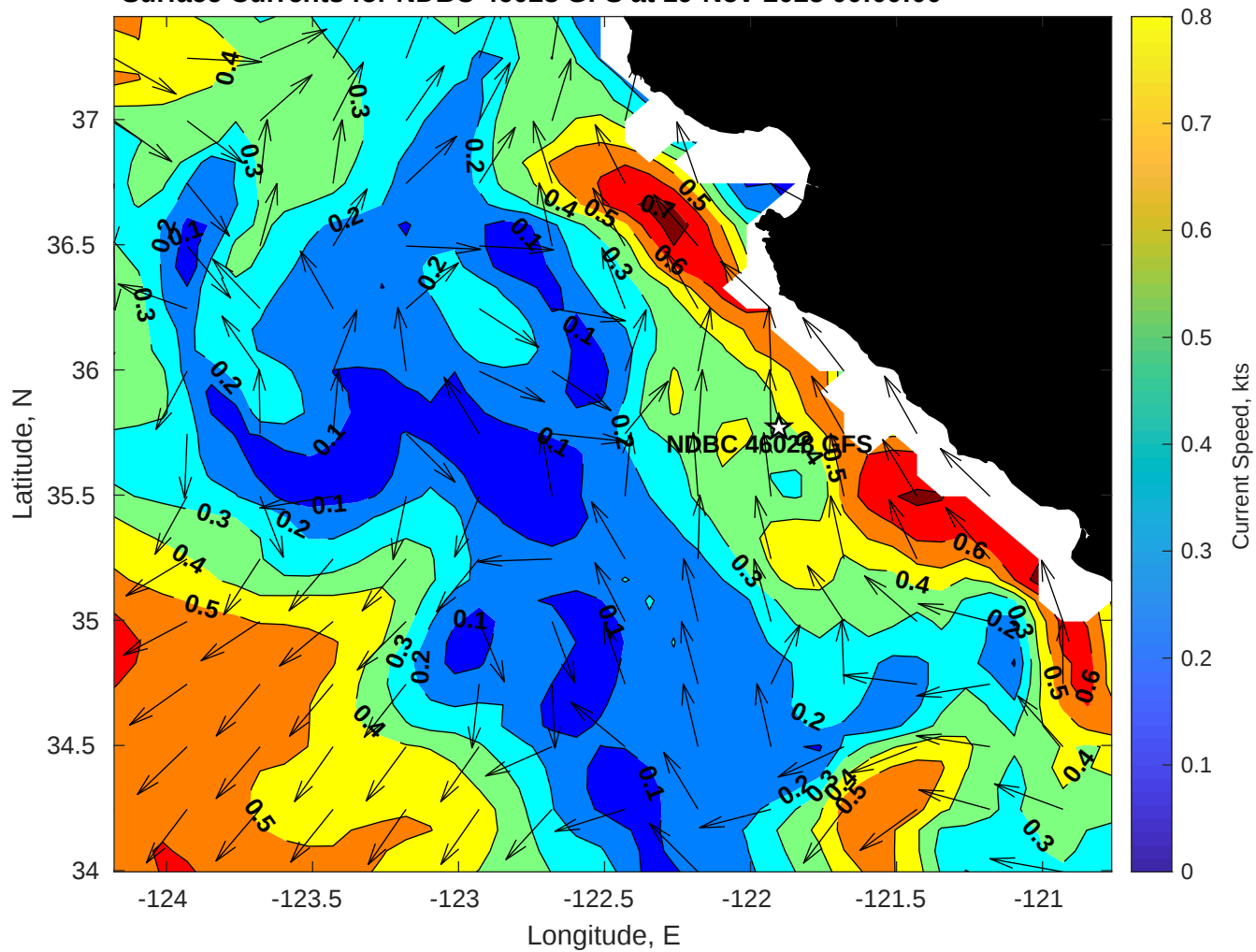
Surface Currents for NDBC 46028 GFS at 19-Nov-2025 00:00:00
