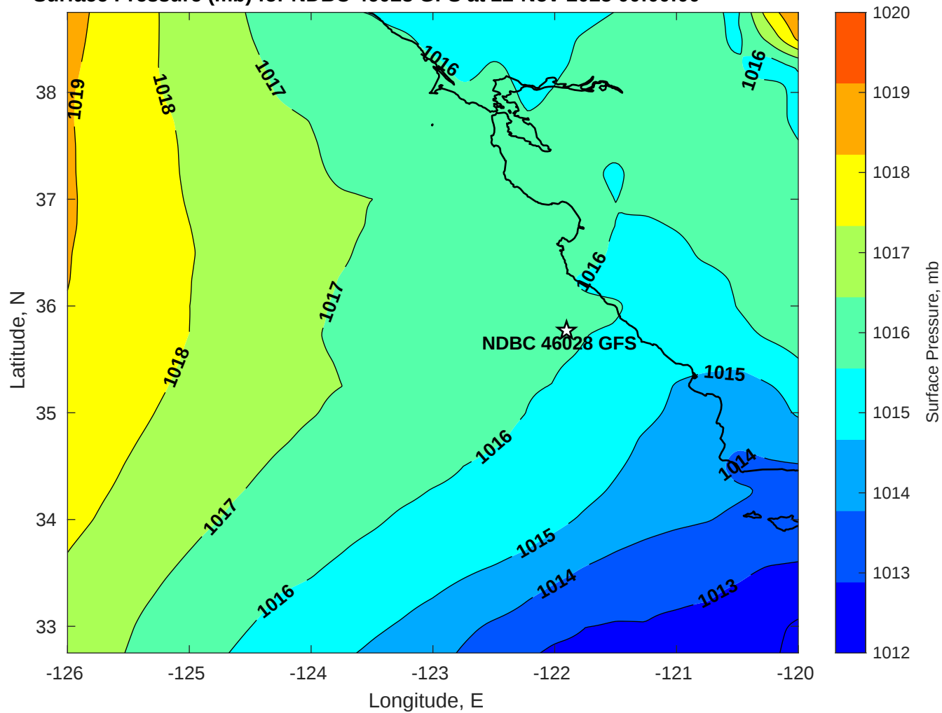
Surface Pressure (mb) for NDBC 46028 GFS at 22-Nov-2025 00:00:00
