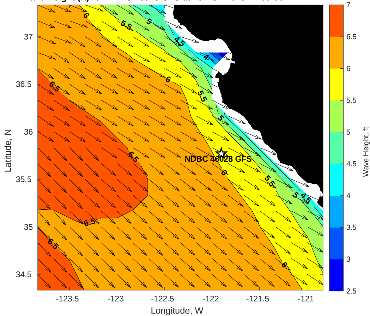
Wave Height (ft) for NDBC 46028 GFS at 19-Nov-2025 21:00:00
