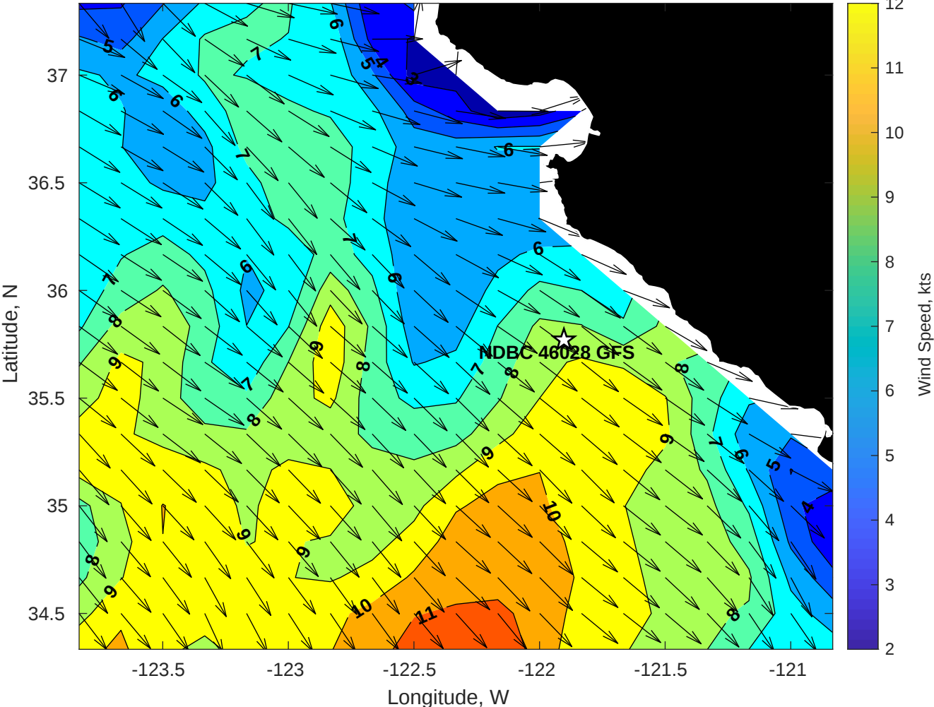
Winds (kts) for NDBC 46028 GFS at 19-Nov-2025 21:00:00
