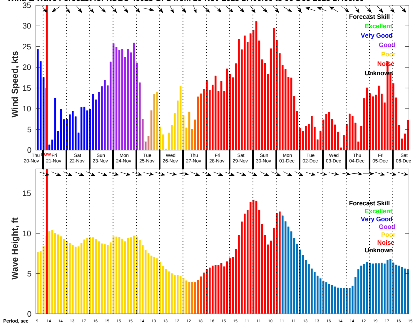
Wind & Wave Forecast for NDBC 46028 GFS from 20-Nov-2025 17:00:00 to 06-Dec-2025 17:00:00
