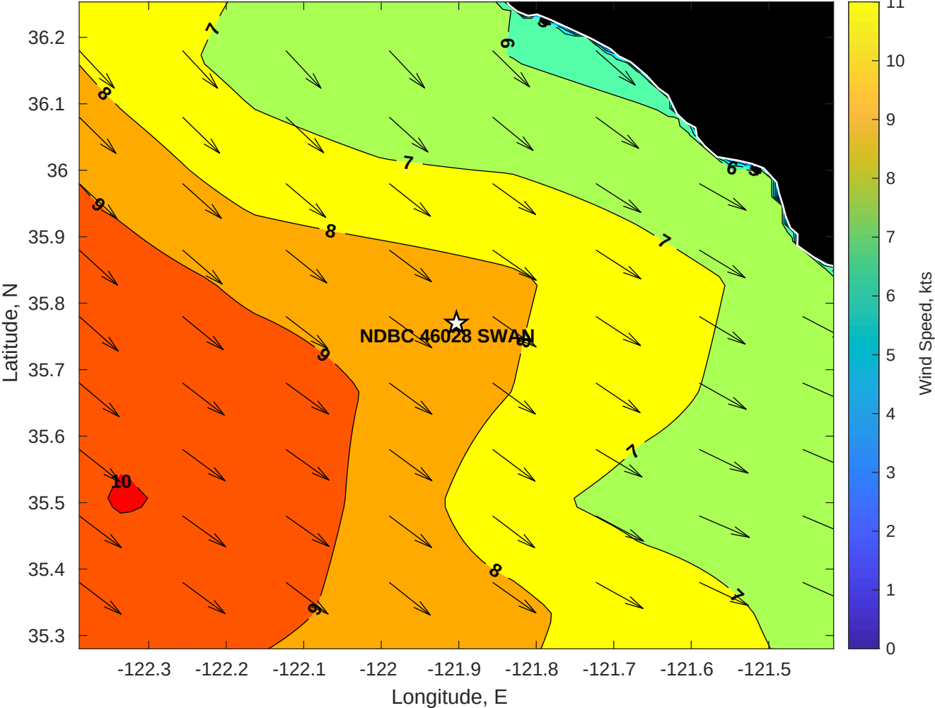
Winds (kts) for NDBC 46028 SWAN at 19-Nov-2025 22:00:00
