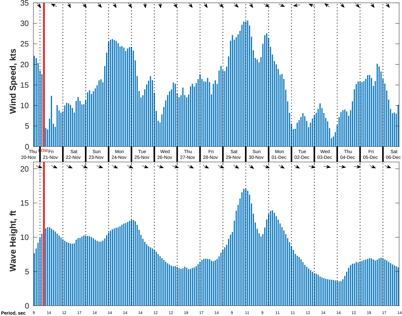
Wind & Wave Forecast for NDBC 46028 SWAN from 20-Nov-2025 17:00:00 to 06-Dec-2025 17:00:00
