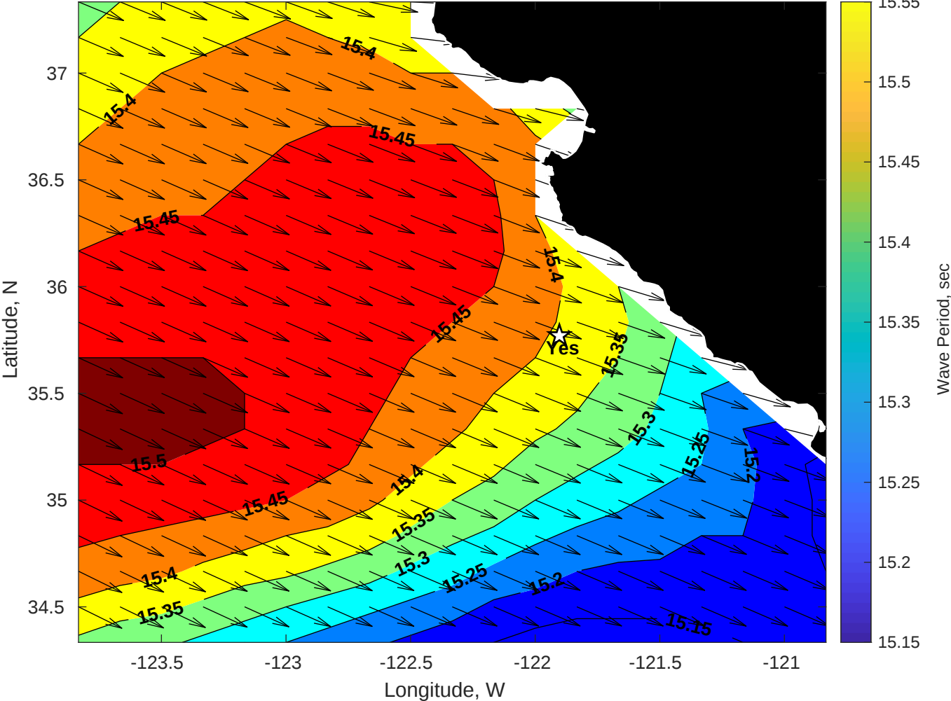
GFS Wave Period (sec) for Yes at 24-Nov-2025 09:00:00
