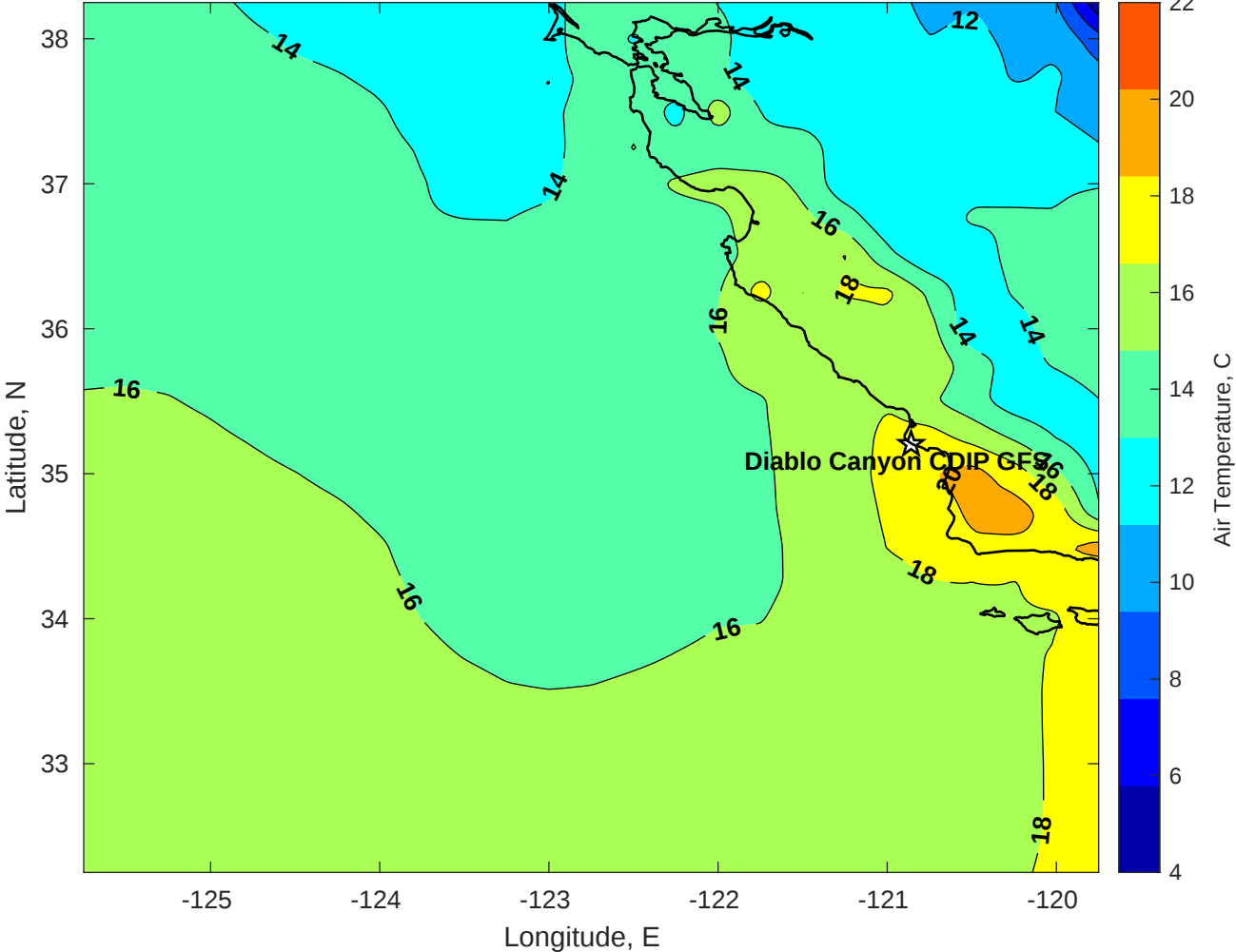
Air Temperature (C) for Diablo Canyon CDIP GFS at 26-Nov-2025
