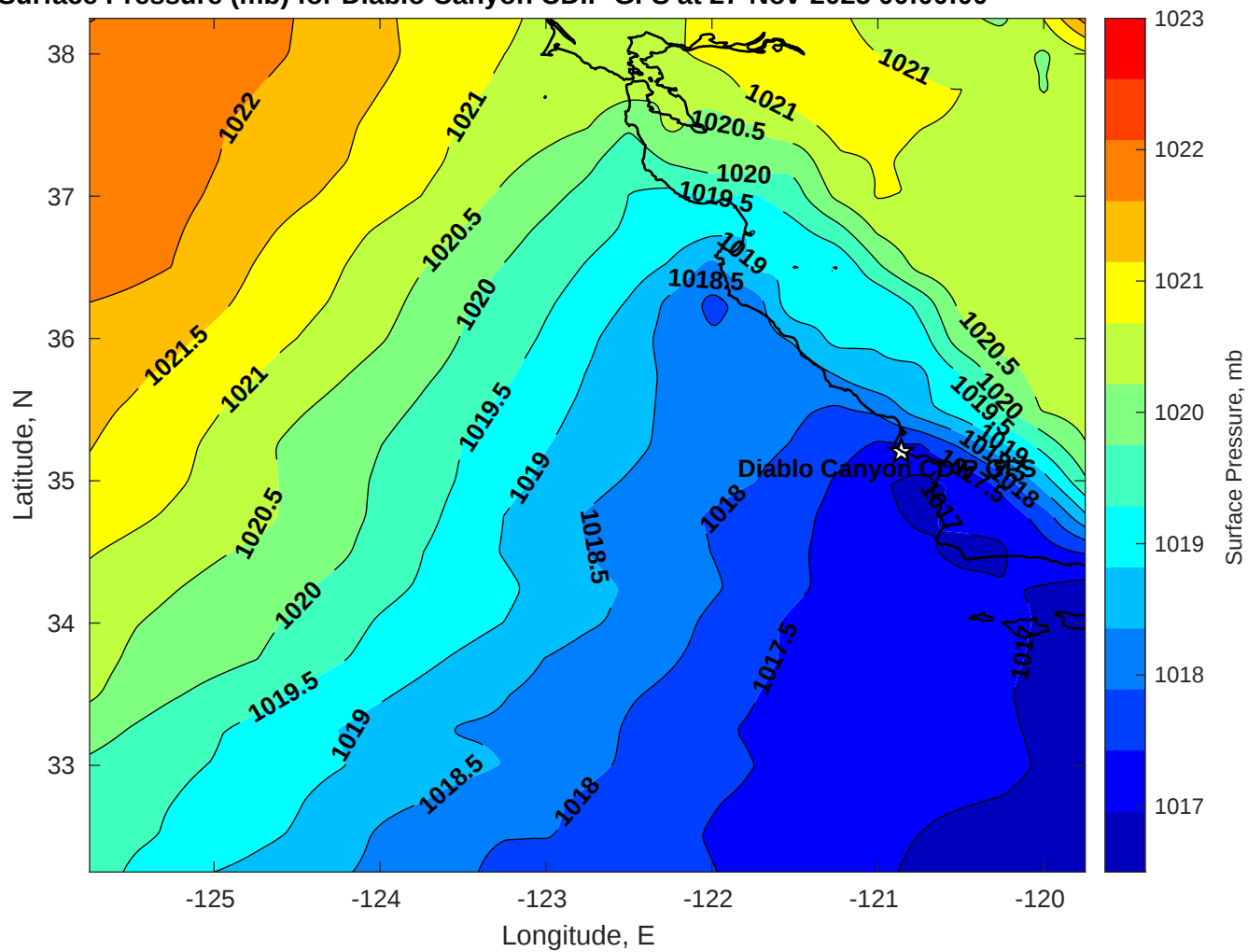
Surface Pressure (mb) for Diablo Canyon CDIP GFS at 27-Nov-2025 00:00:00
