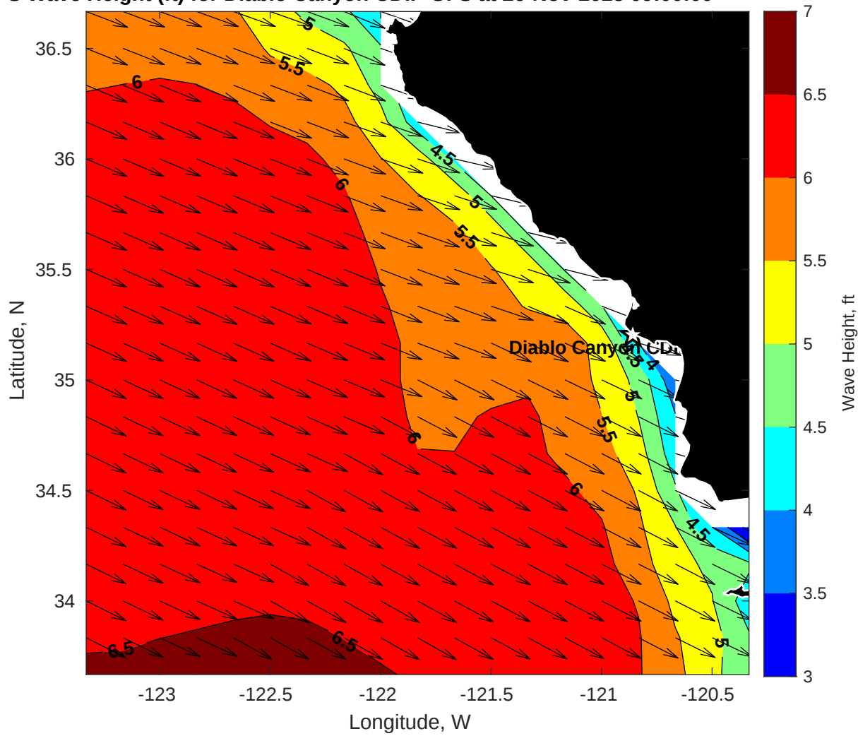
GFS Wave Height (ft) for Diablo Canyon CDIP GFS at 26-Nov-2025 09:00:00
