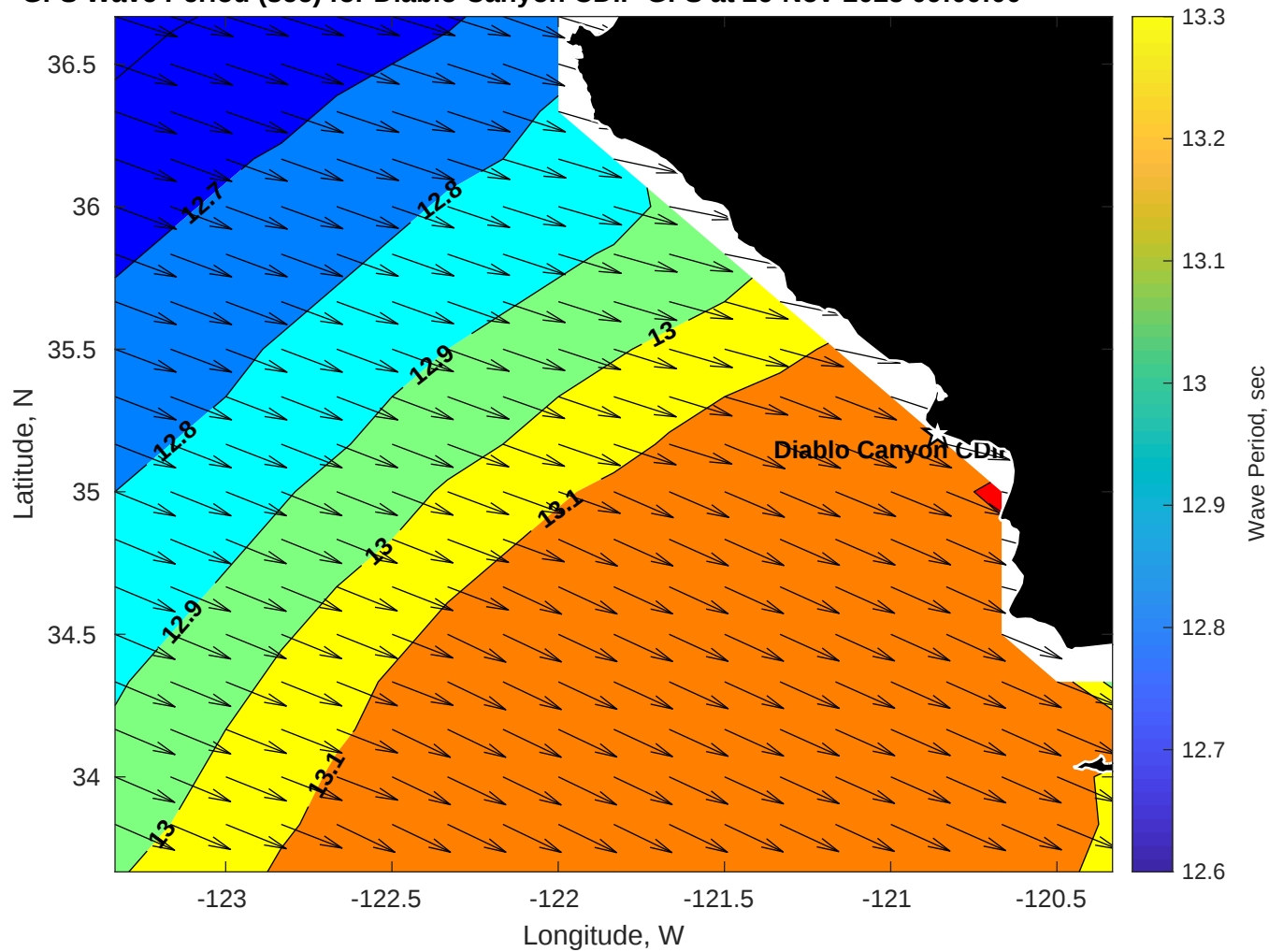
GFS Wave Period (sec) for Diablo Canyon CDIP GFS at 26-Nov-2025 09:00:00
