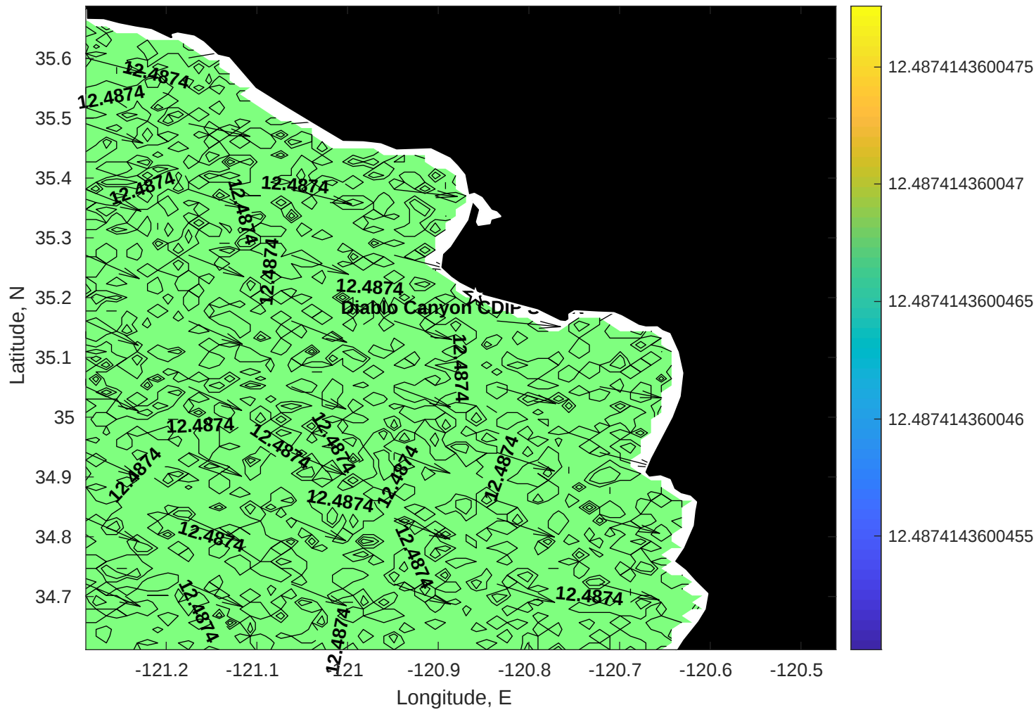
SWAN Wave Period (sec) for Diablo Canyon CDIP SWAN at 26-Nov-2025 10:00:00
