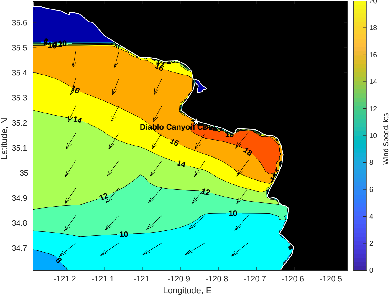
SWAN Winds (kts) for Diablo Canyon CDIP SWAN at 26-Nov-2025 10:00:00
