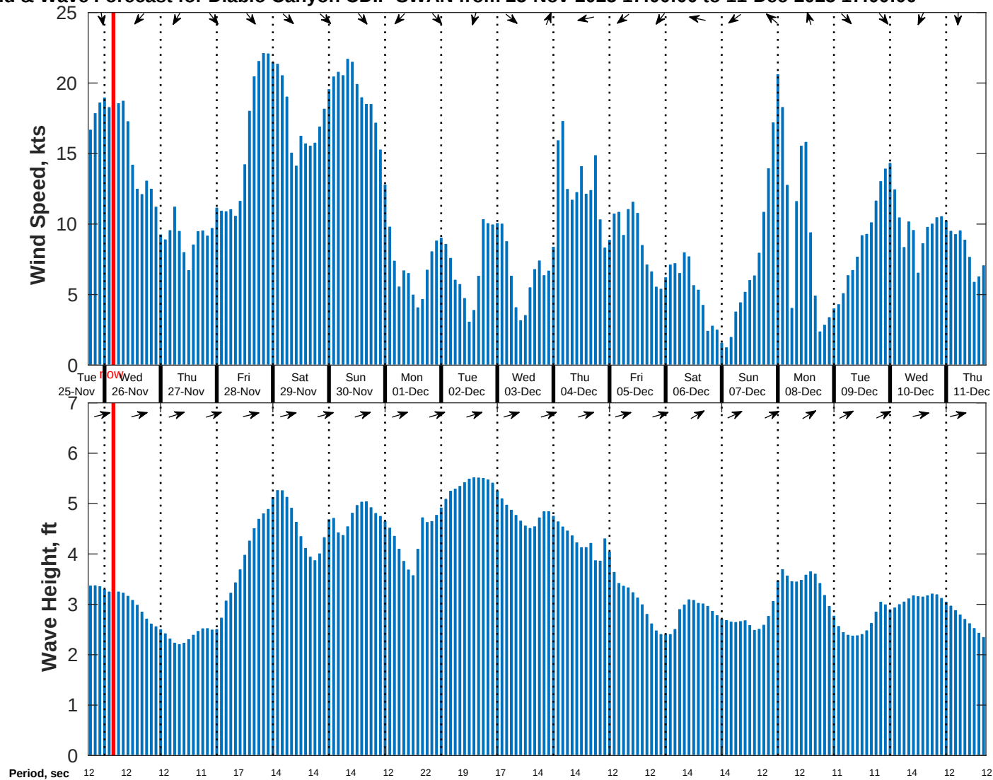
Wind & Wave Forecast for Diablo Canyon CDIP SWAN from 25-Nov-2025 17:00:00 to 11-Dec-2025 17:00:00
