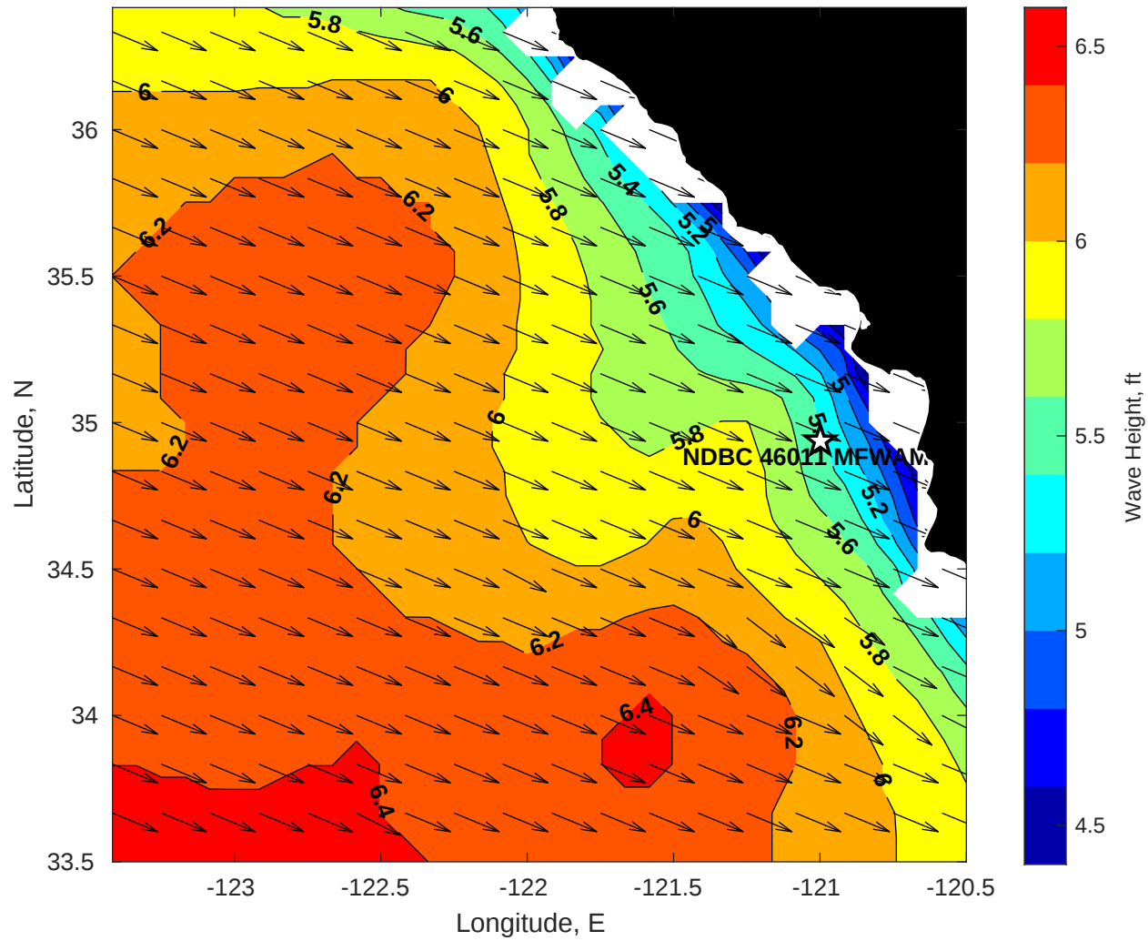
WAM Wave Height (ft) for NDBC 46011 MFWAM at 26-Nov-2025 09:00:00
