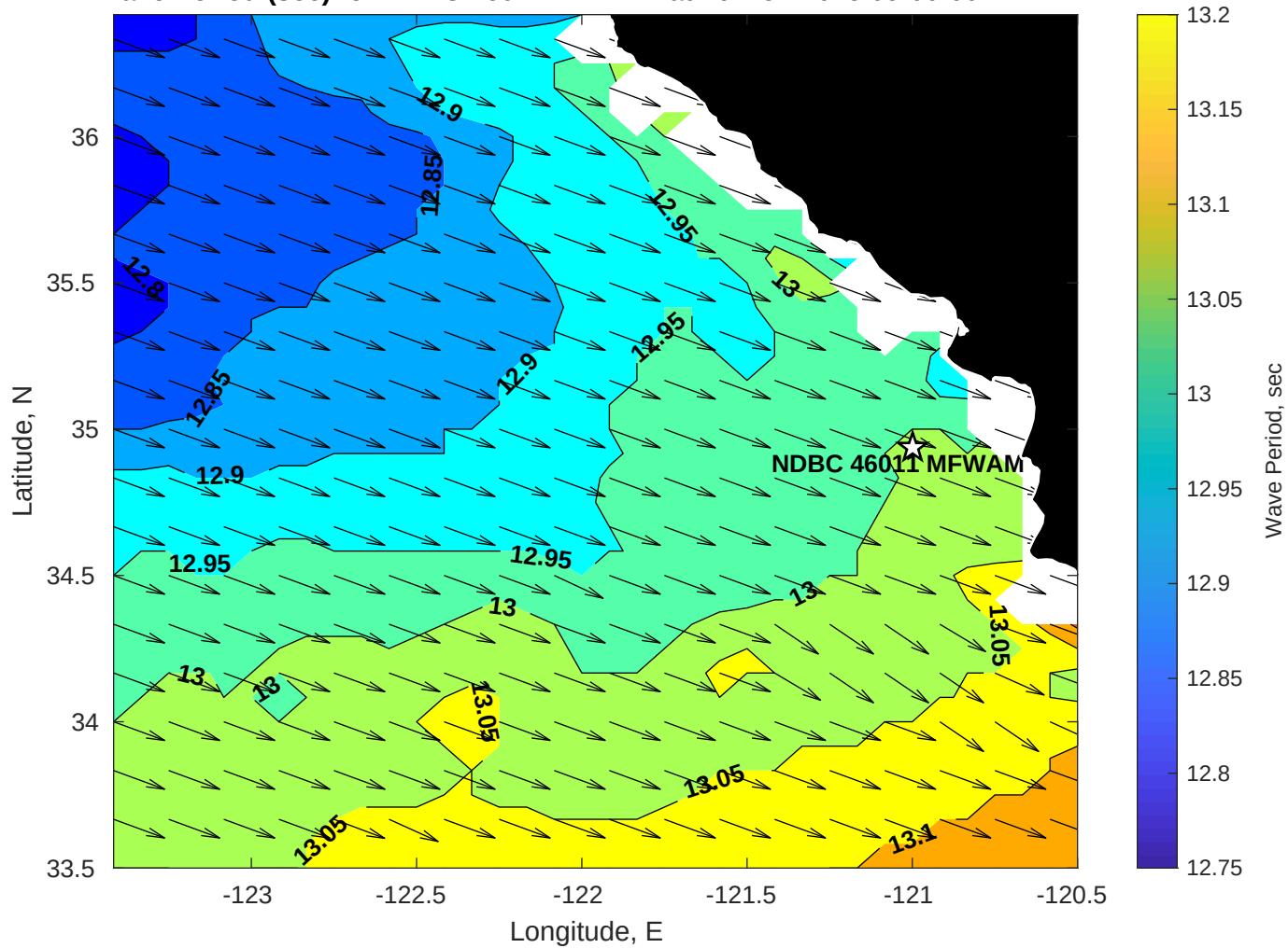
WAM Wave Period (sec) for NDBC 46011 MFWAM at 26-Nov-2025 09:00:00
