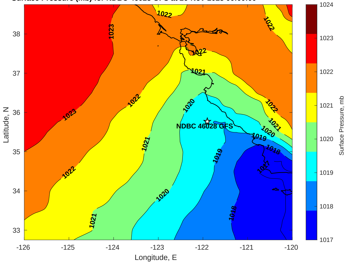
Surface Pressure (mb) for NDBC 46028 GFS at 26-Nov-2025 00:00:00
