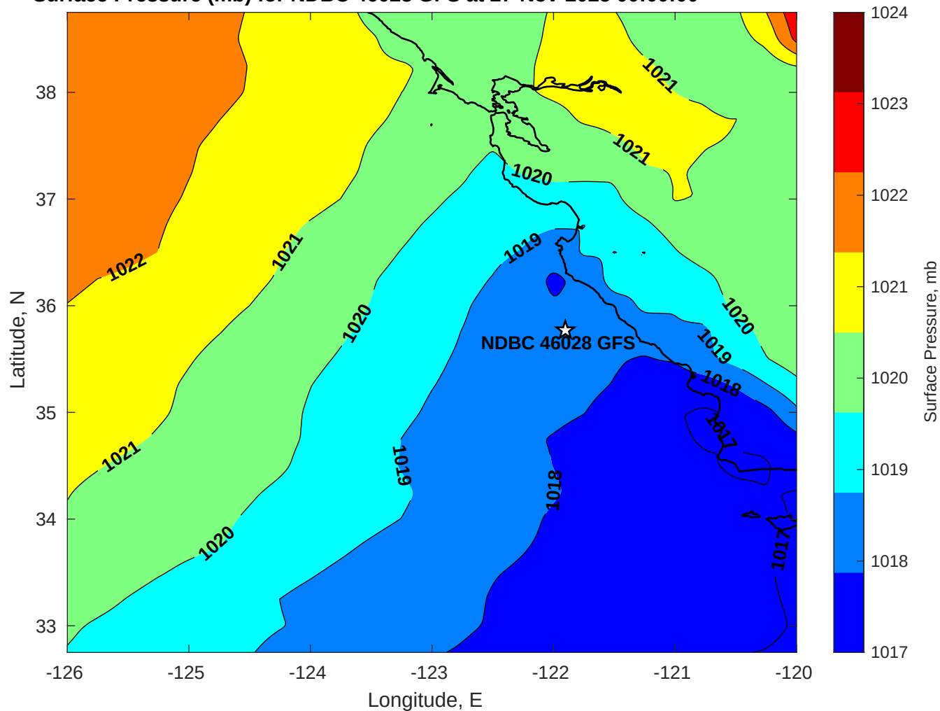
Surface Pressure (mb) for NDBC 46028 GFS at 27-Nov-2025 00:00:00
