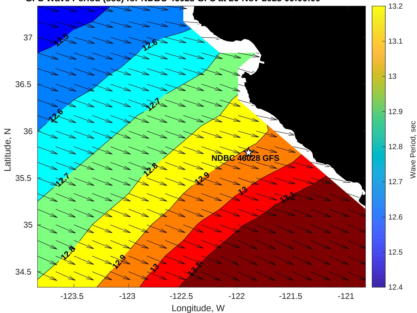
GFS Wave Period (sec) for NDBC 46028 GFS at 26-Nov-2025 09:00:00
