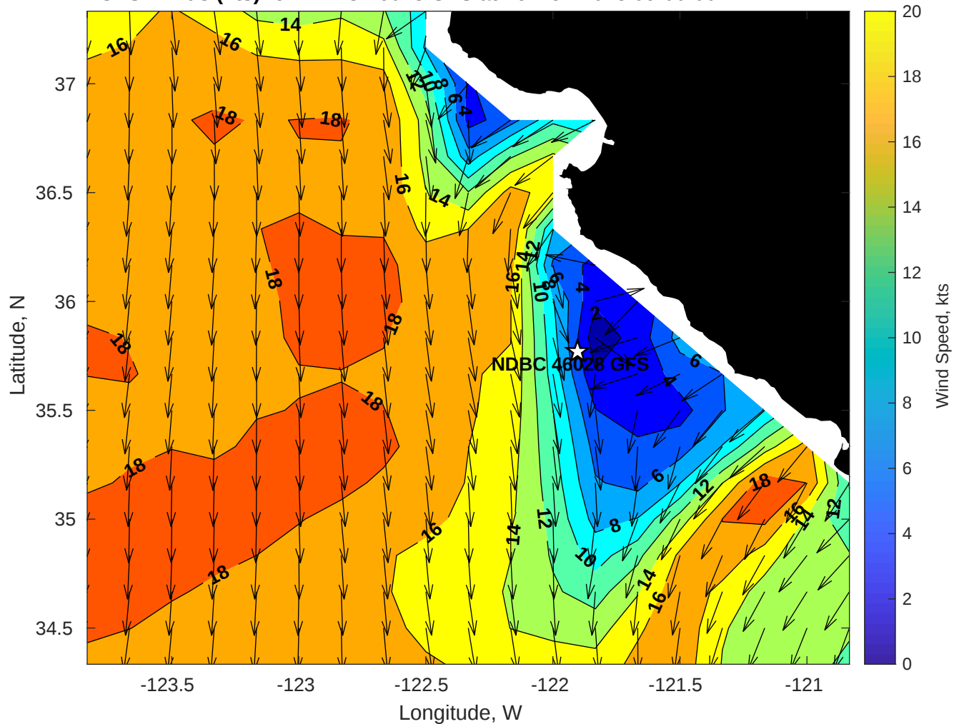
GFS Winds (kts) for NDBC 46028 GFS at 26-Nov-2025 09:00:00
