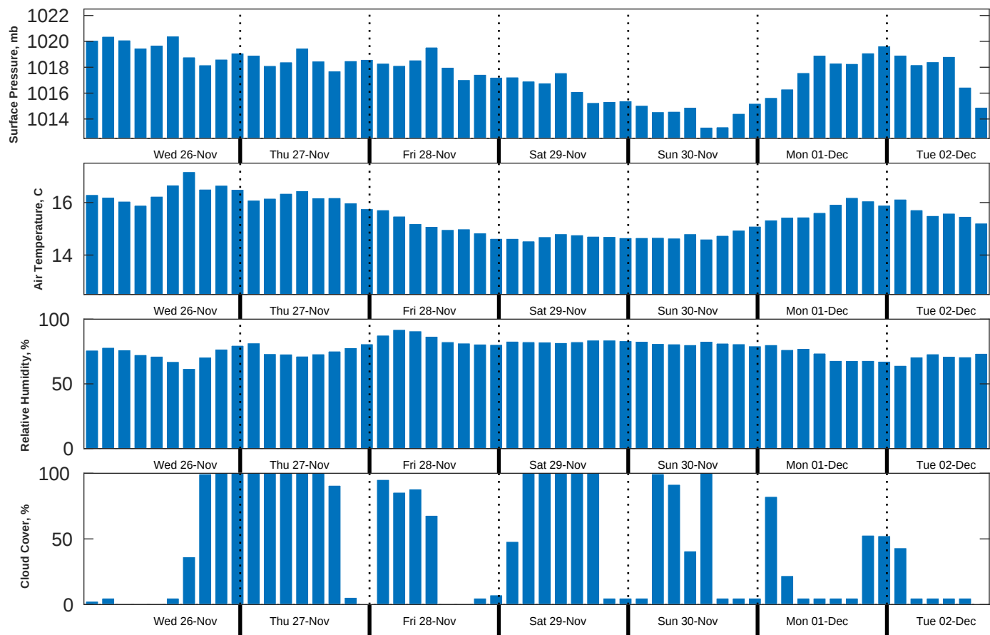
Met Forecast for NDBC 46028 GFS from 26-Nov-2025 00:00:00 to 03-Dec-2025 00:00:00
