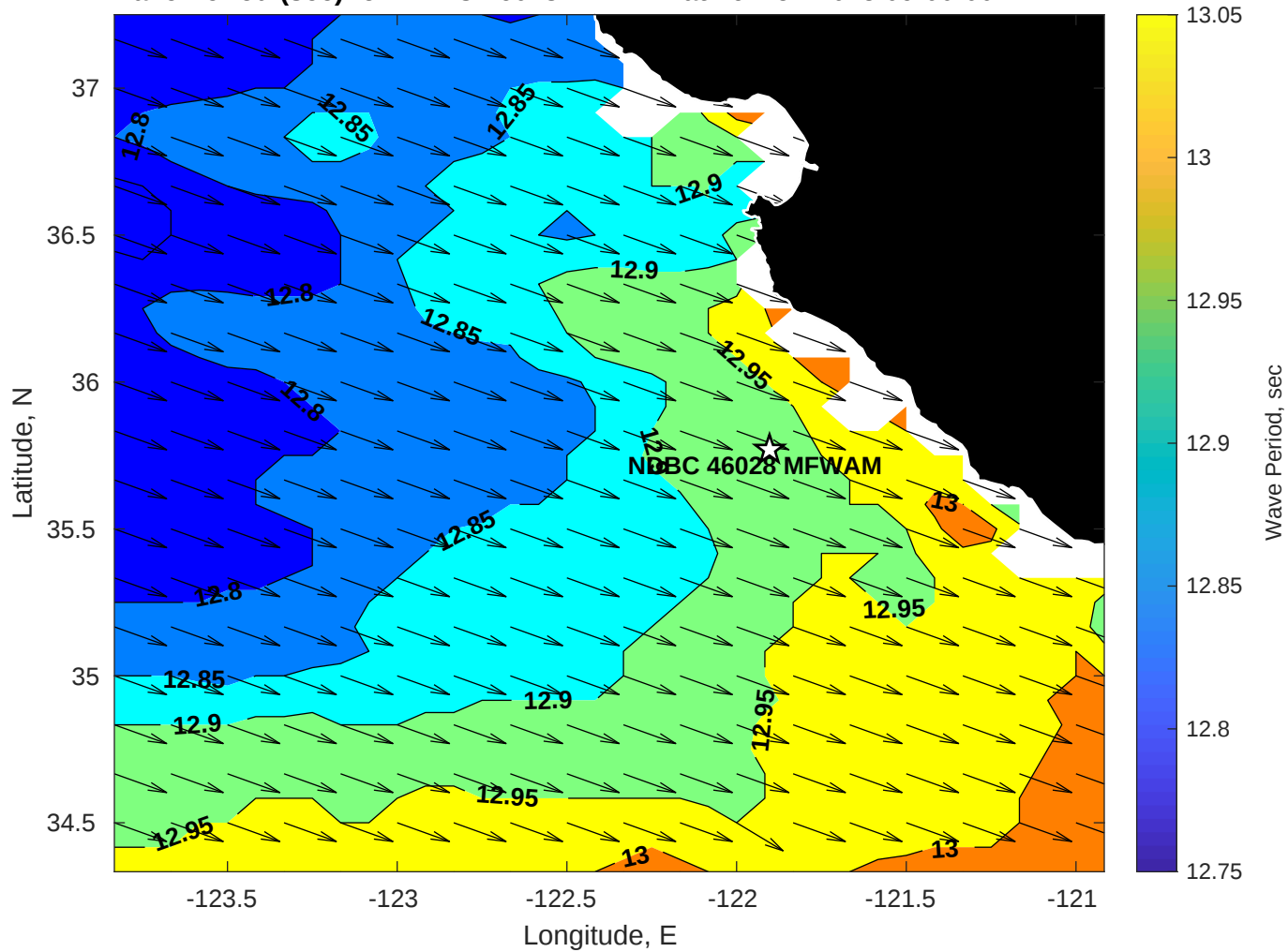
WAM Wave Period (sec) for NDBC 46028 MFWAM at 26-Nov-2025 09:00:00
