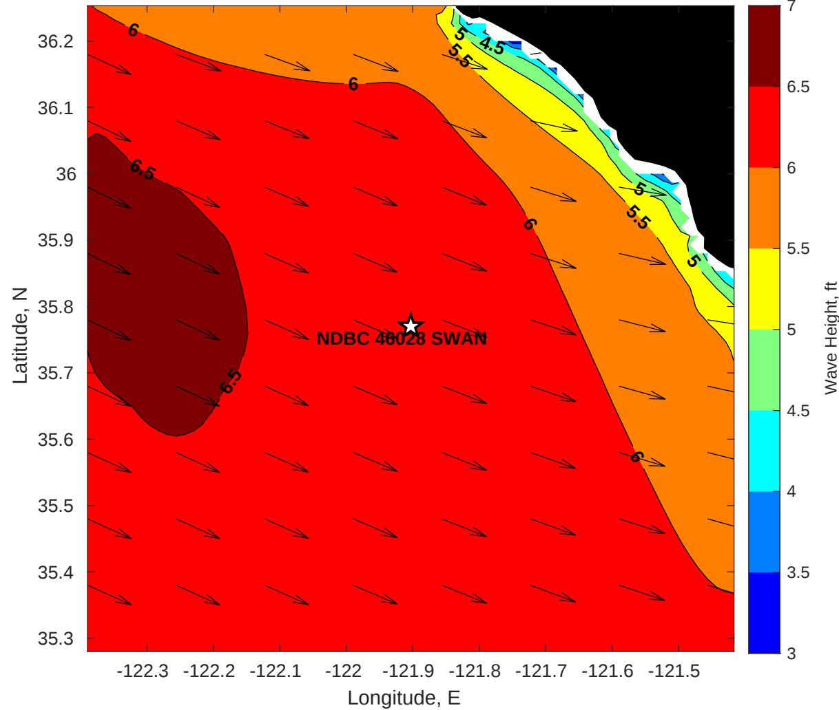
SWAN Wave Height (ft) for NDBC 46028 SWAN at 26-Nov-2025 10:00:00
