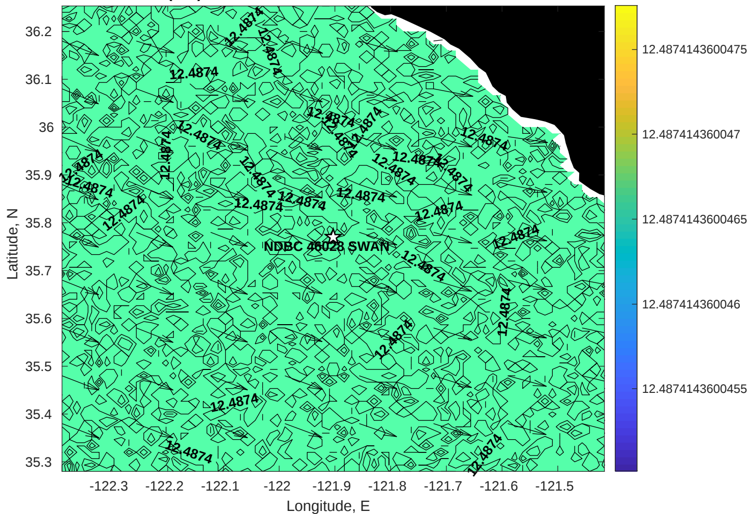
SWAN Wave Period (sec) for NDBC 46028 SWAN at 26-Nov-2025 10:00:00
