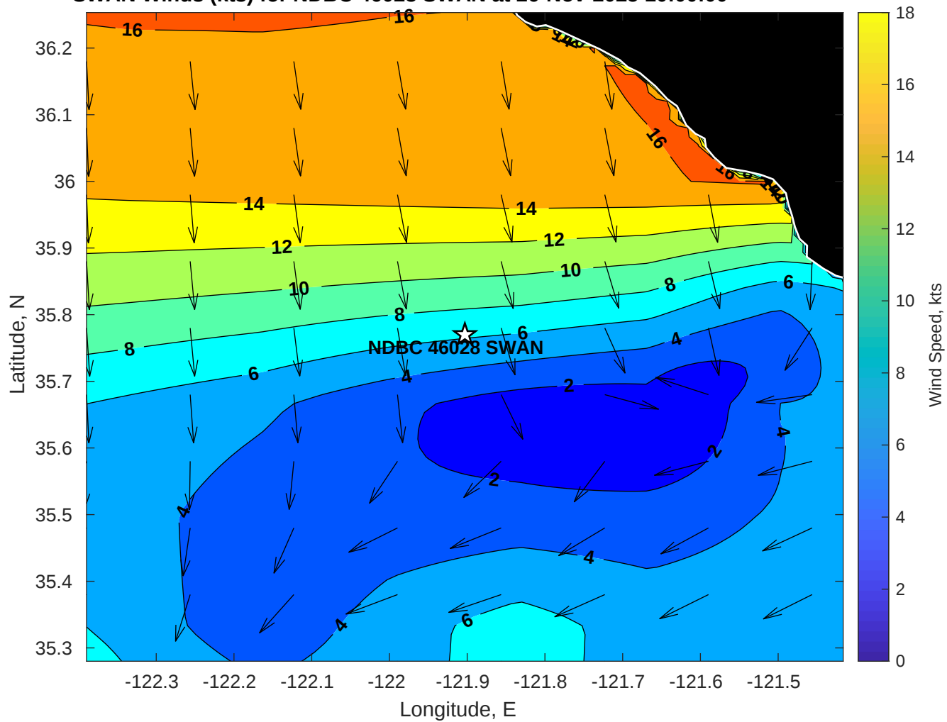
SWAN Winds (kts) for NDBC 46028 SWAN at 26-Nov-2025 10:00:00
