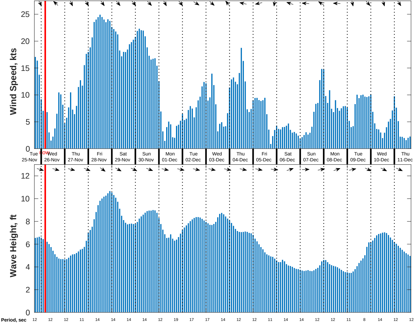
Wind & Wave Forecast for NDBC 46028 SWAN from 25-Nov-2025 17:00:00 to 11-Dec-2025 17:00:00
