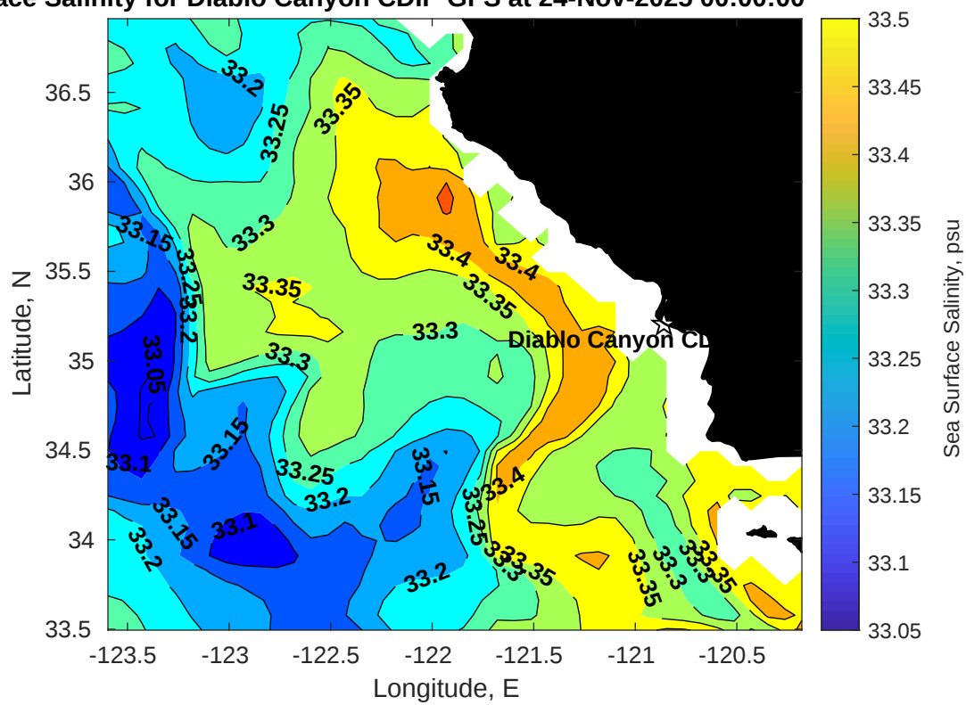
Surface Salinity for Diablo Canyon CDIP GFS at 24-Nov-2025 00:00:00
