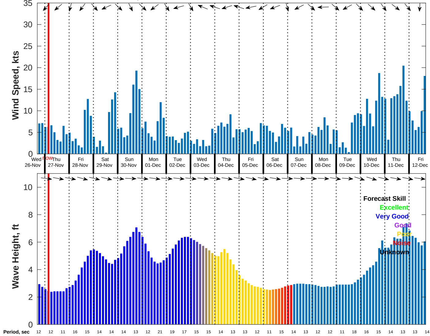
Wind & Wave Forecast for Diablo Canyon CDIP GFS from 26-Nov-2025 17:00:00 to 12-Dec-2025 17:00:00
