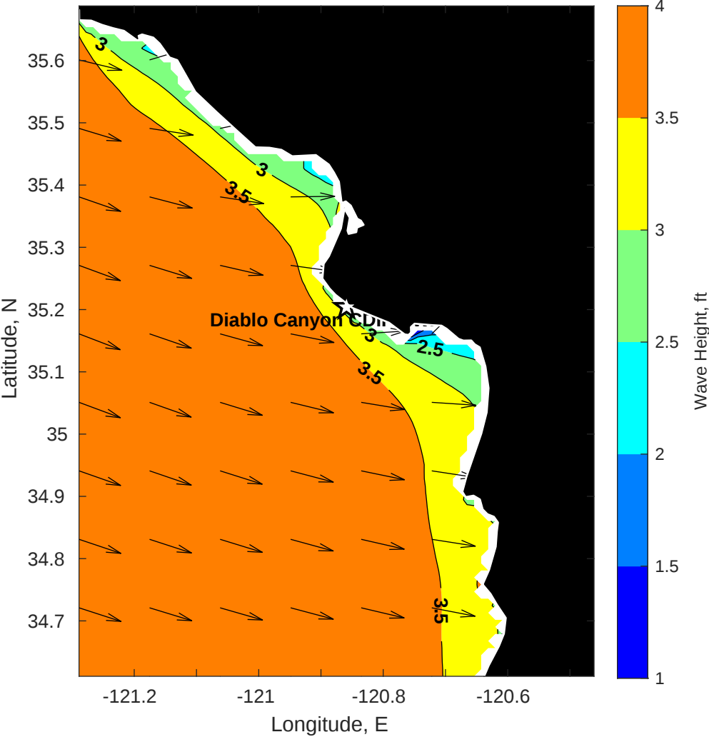
SWAN Wave Height (ft) for Diablo Canyon CDIP SWAN at 27-Nov-2025 10:00:00
