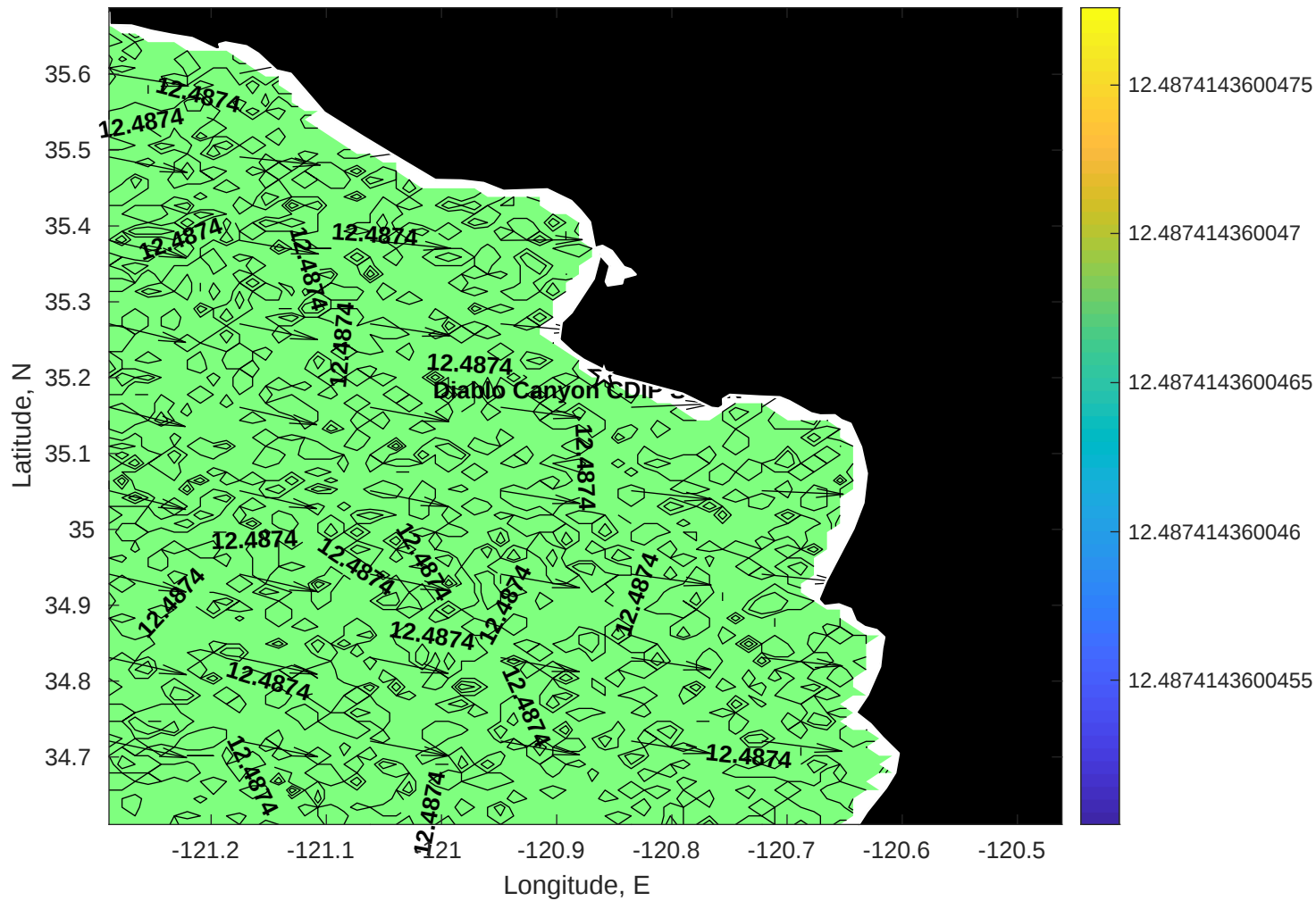
SWAN Wave Period (sec) for Diablo Canyon CDIP SWAN at 27-Nov-2025 10:00:00
