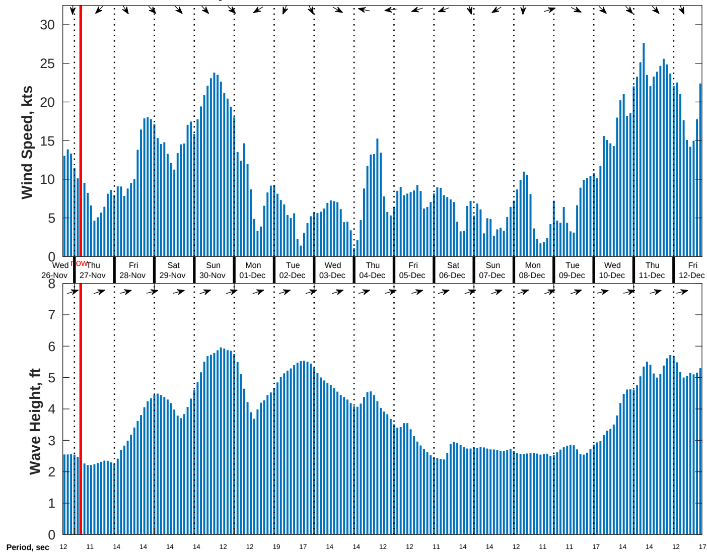
Wind & Wave Forecast for Diablo Canyon CDIP SWAN from 26-Nov-2025 17:00:00 to 12-Dec-2025 17:00:00
