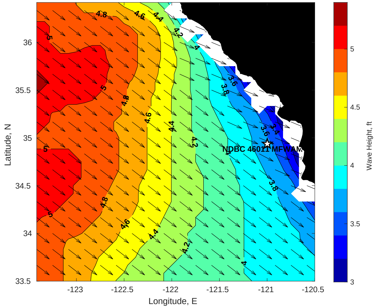
WAM Wave Height (ft) for NDBC 46011 MFWAM at 27-Nov-2025 09:00:00
