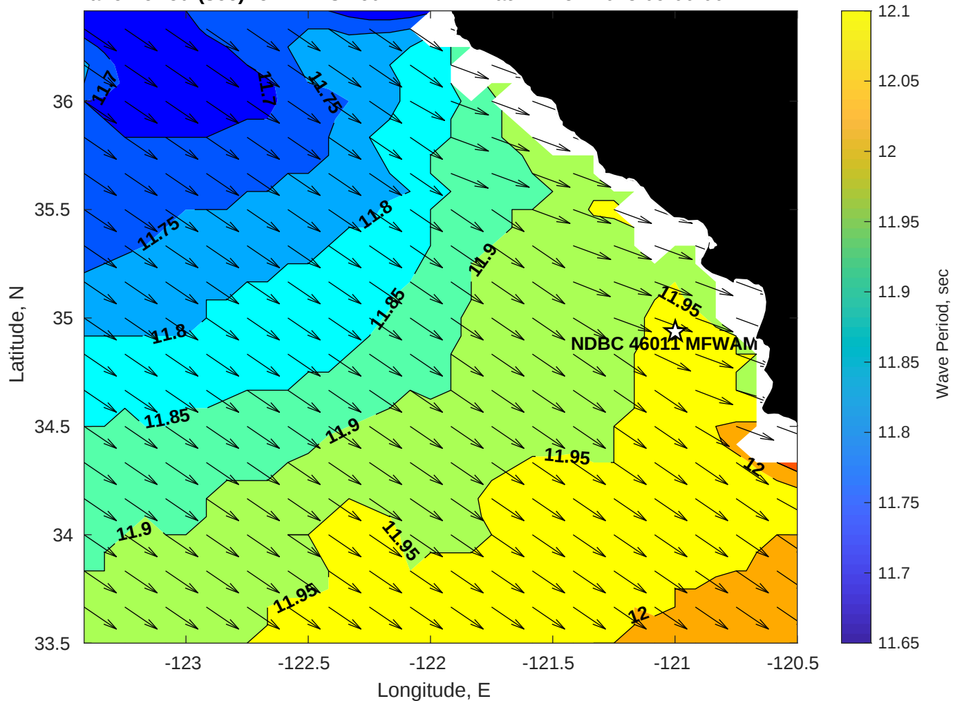
WAM Wave Period (sec) for NDBC 46011 MFWAM at 27-Nov-2025 09:00:00
