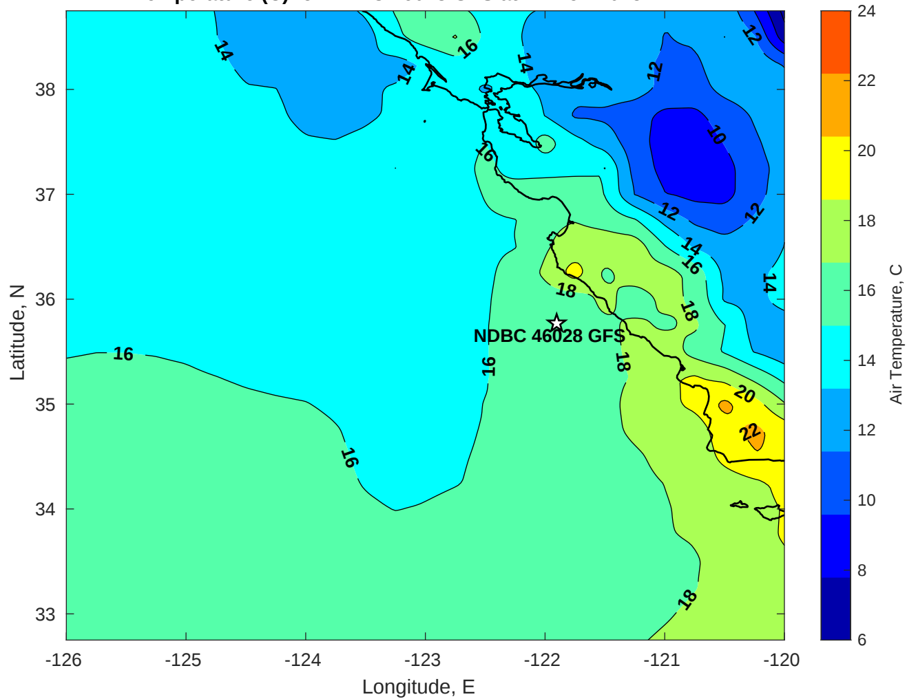
Air Temperature (C) for NDBC 46028 GFS at 27-Nov-2025
