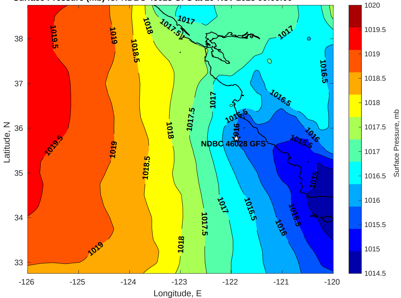
Surface Pressure (mb) for NDBC 46028 GFS at 29-Nov-2025 00:00:00
