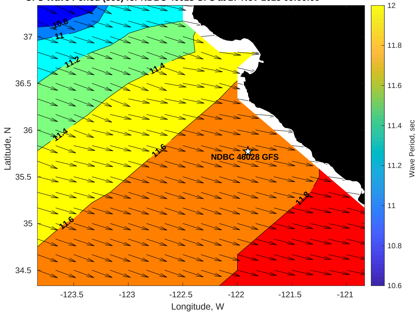
GFS Wave Period (sec) for NDBC 46028 GFS at 27-Nov-2025 09:00:00
