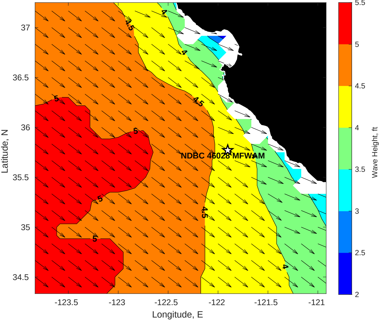
WAM Wave Height (ft) for NDBC 46028 MFWAM at 27-Nov-2025 09:00:00
