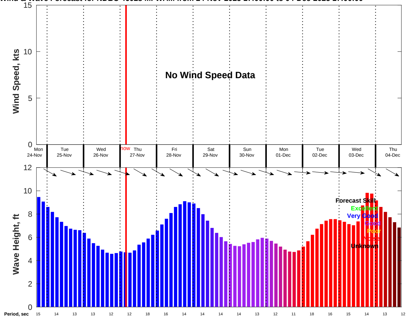
Wind & Wave Forecast for NDBC 46028 MFWAM from 24-Nov-2025 17:00:00 to 04-Dec-2025 17:00:00
