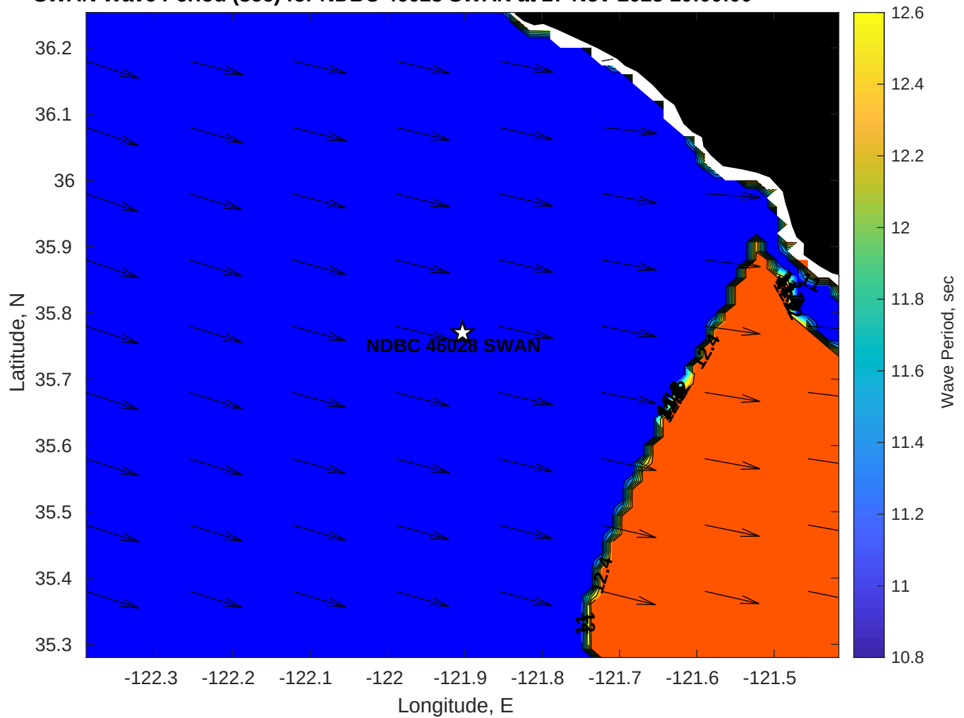
SWAN Wave Period (sec) for NDBC 46028 SWAN at 27-Nov-2025 10:00:00
