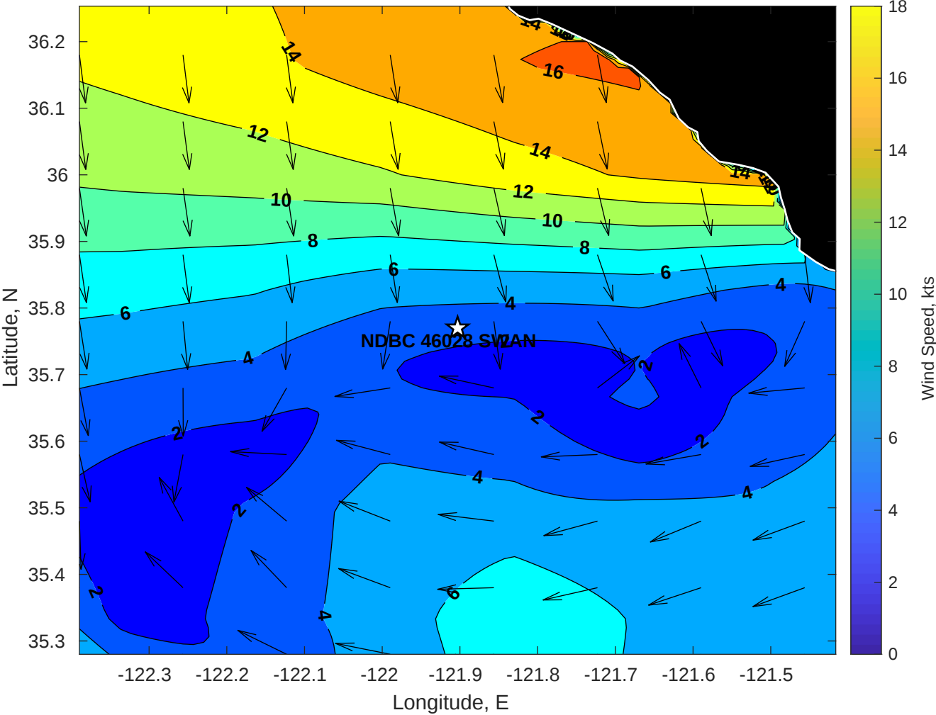
SWAN Winds (kts) for NDBC 46028 SWAN at 27-Nov-2025 10:00:00
