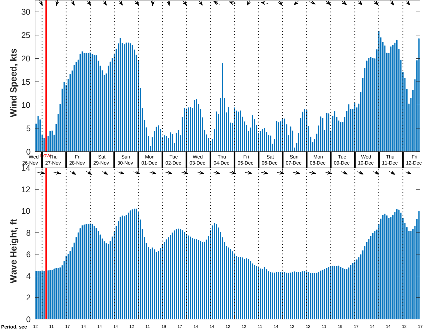
Wind & Wave Forecast for NDBC 46028 SWAN from 26-Nov-2025 17:00:00 to 12-Dec-2025 17:00:00
