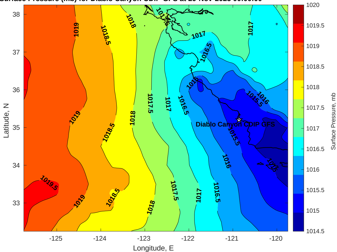
Surface Pressure (mb) for Diablo Canyon CDIP GFS at 29-Nov-2025 00:00:00
