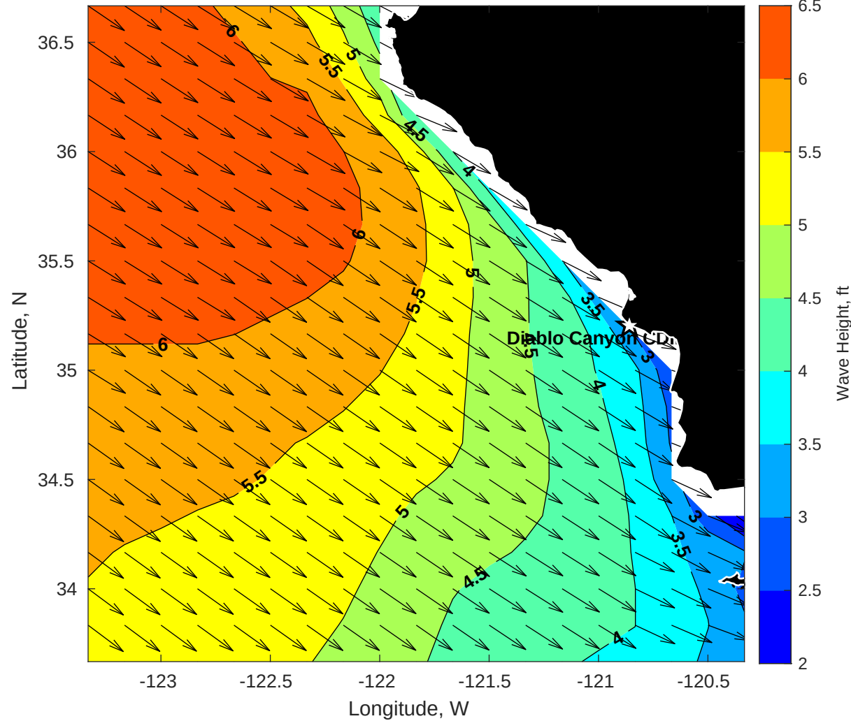
GFS Wave Height (ft) for Diablo Canyon CDIP GFS at 28-Nov-2025 09:00:00
