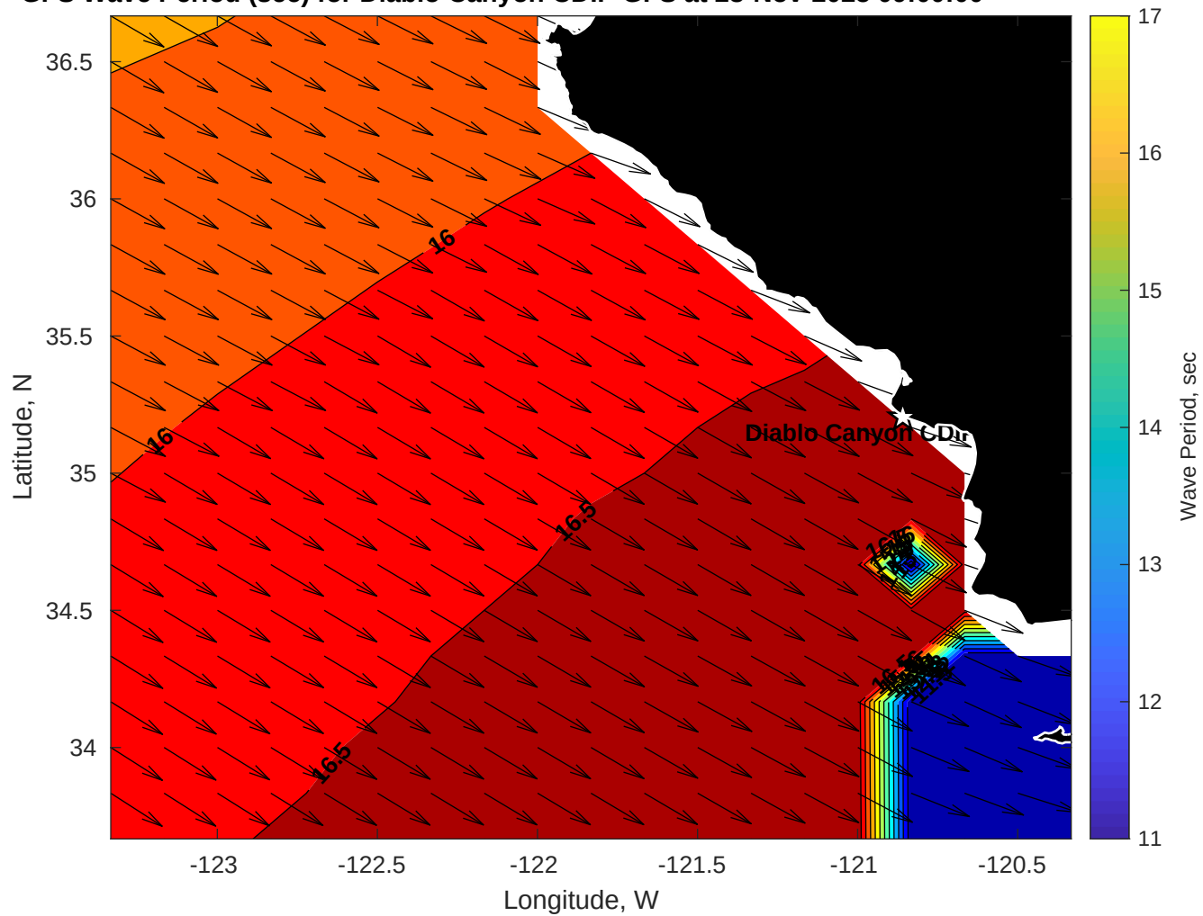
GFS Wave Period (sec) for Diablo Canyon CDIP GFS at 28-Nov-2025 09:00:00
